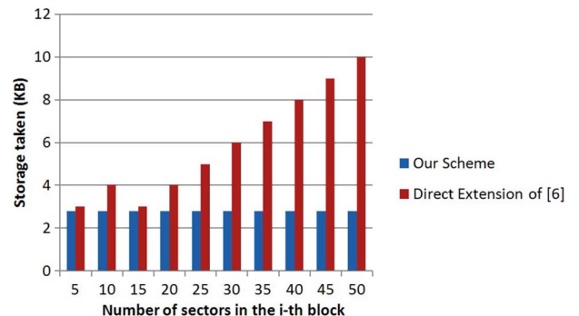
Fig. 8. Comparison of the total storage overhead invoked by 10 * 280 -byte insertions to the i -th block in our scheme, as opposed to the direct extension of [6].
