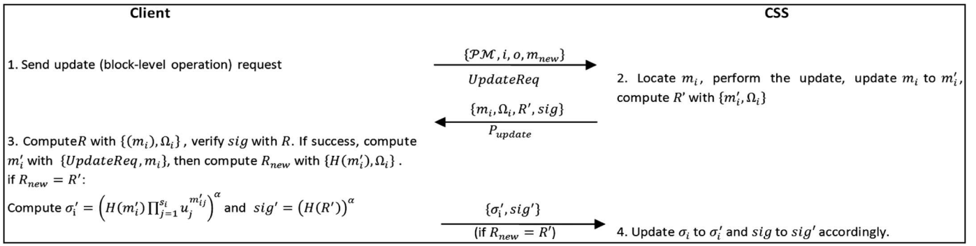
Fig. 3. Verifiable PM-typed Data Update in our scheme.
