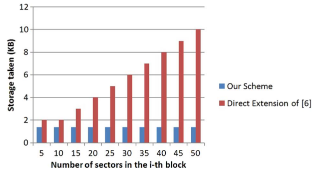
Fig. 7. Comparison of the total storage overhead invoked by 10 * 140 -byte insertions to the i -th block in our scheme, as opposed to the direct extension of [6].
